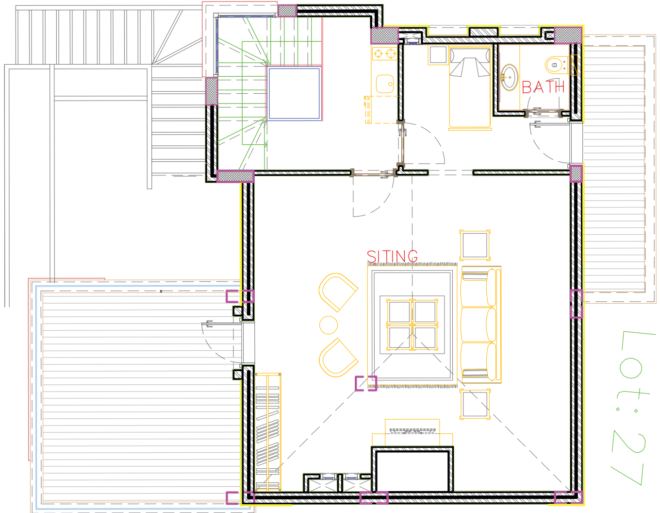
Villa 27 Attic plan
