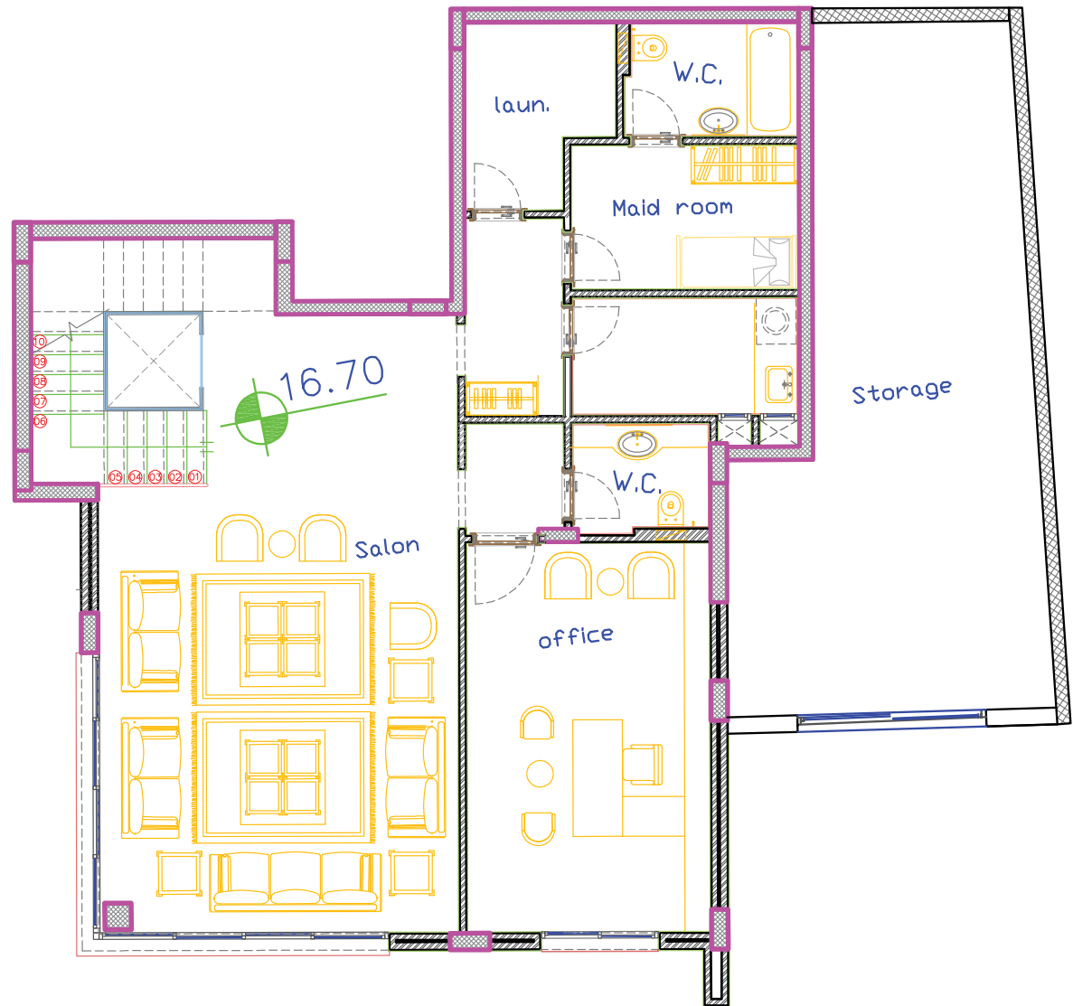
Villa 27 Basement Plan
